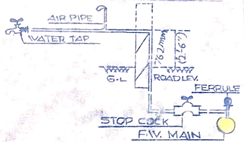
DETAILS OF FEEDING POINT
